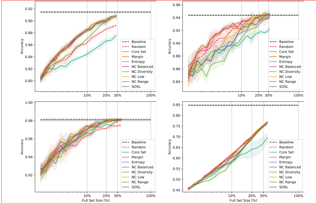
Figure 1: Classification accuracy over training set size for all strategies on Fashion-MNIST (top left), TSR (top right), MNIST (bottom left) and CIFAR10 (bottom right). The plotted value is the median of five runs and the shaded area denotes one standard deviation.
