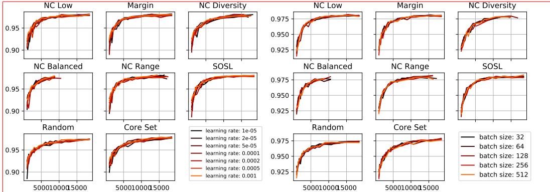
Figure 2: Changes in learning rate (left) and batch size (right) for various Active Learning strategies on MNIST. The plotted value is the median of five runs.
