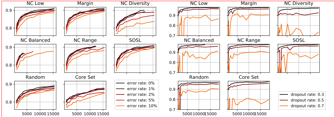
Figure 3: Active Learning strategy results for various synthetic labelling error rates on Fashion-MNIST (left) and different dropout regularization rates on MNIST (right). The plotted value is the median of five runs.
