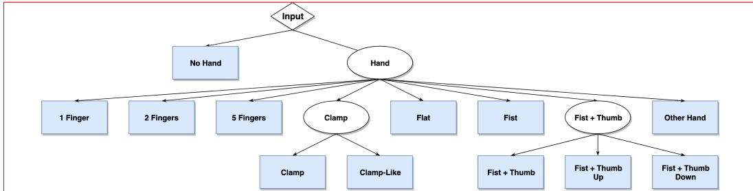
Figure 6: Hierarchical labels for hand gesture recognition. Blue boxes denote the 12 classes.
