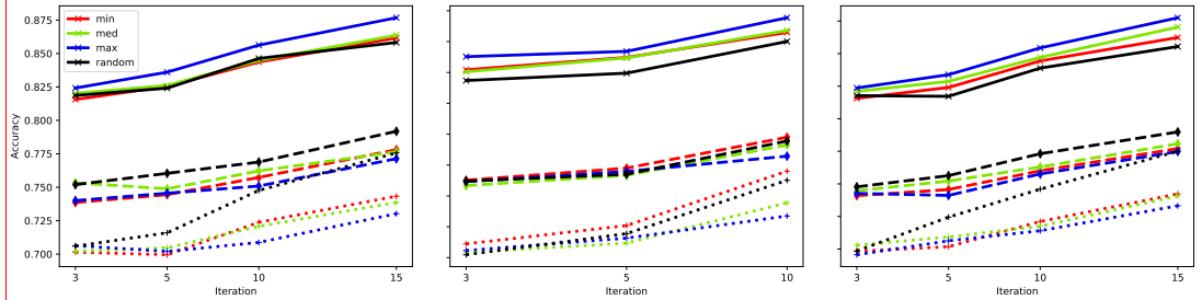
Figure 3: Active Learning strategy results for various synthetic labelling error rates on Fashion-MNIST (left) and different dropout regularization rates on MNIST (right). The plotted value is the median of five runs.
